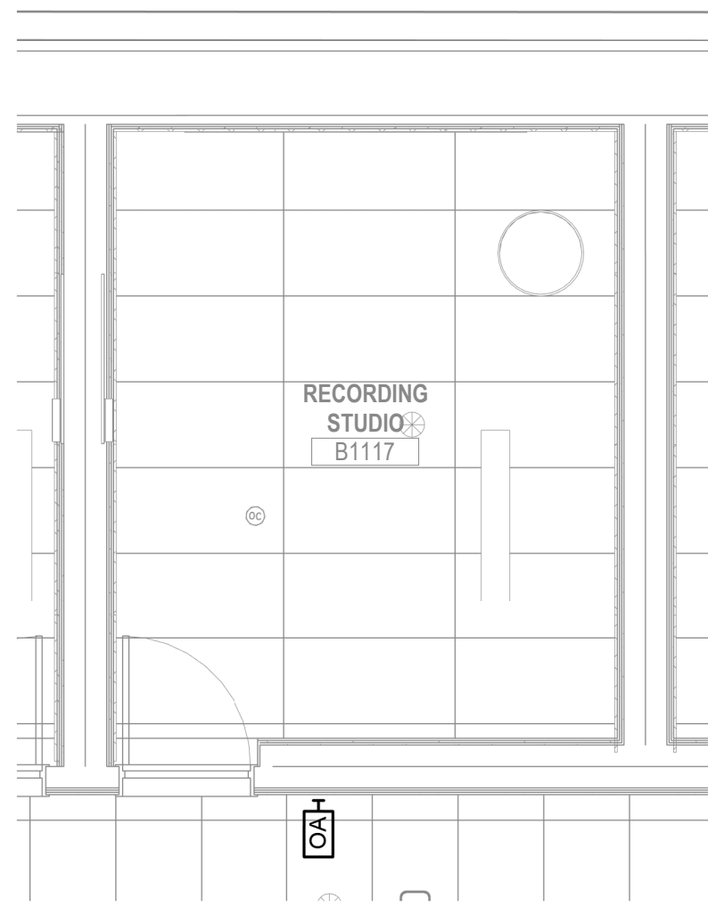
9 RECORDING STUDIO B1117 - ENLARGED RCP - ADDITIVE BID ALTERNATE (RECORDING STUDIO) 1/4" = 1'-0"
