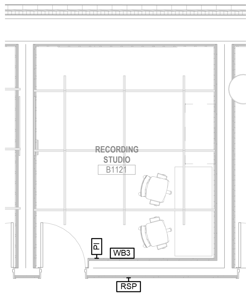
10 RECORDING STUDIO B1121 - ENLARGED PLAN - ADDITIVE BID ALTERNATE (RECORDING STUDIO) 1/4" = 1'-0"
