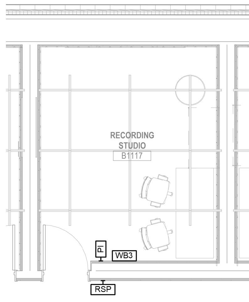
8 RECORDING STUDIO B1117 - ENLARGED PLAN - ADDITIVE BID ALTERNATE (RECORDING STUDIO) 1/4" = 1'-0"
