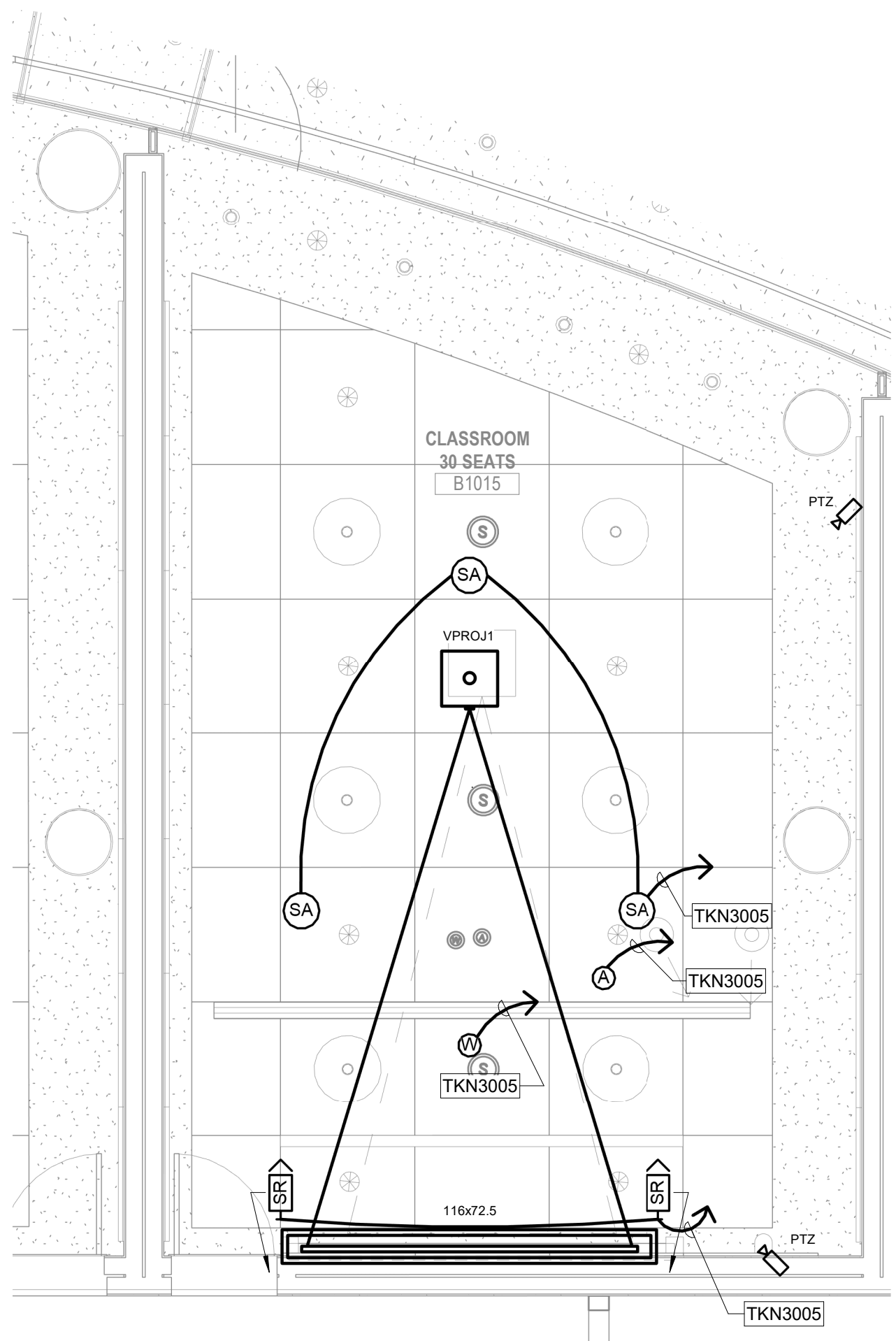
2 CLASSROOM 30 SEATS B1015 - ENLARGED RCP 1/4" = 1'-0"
