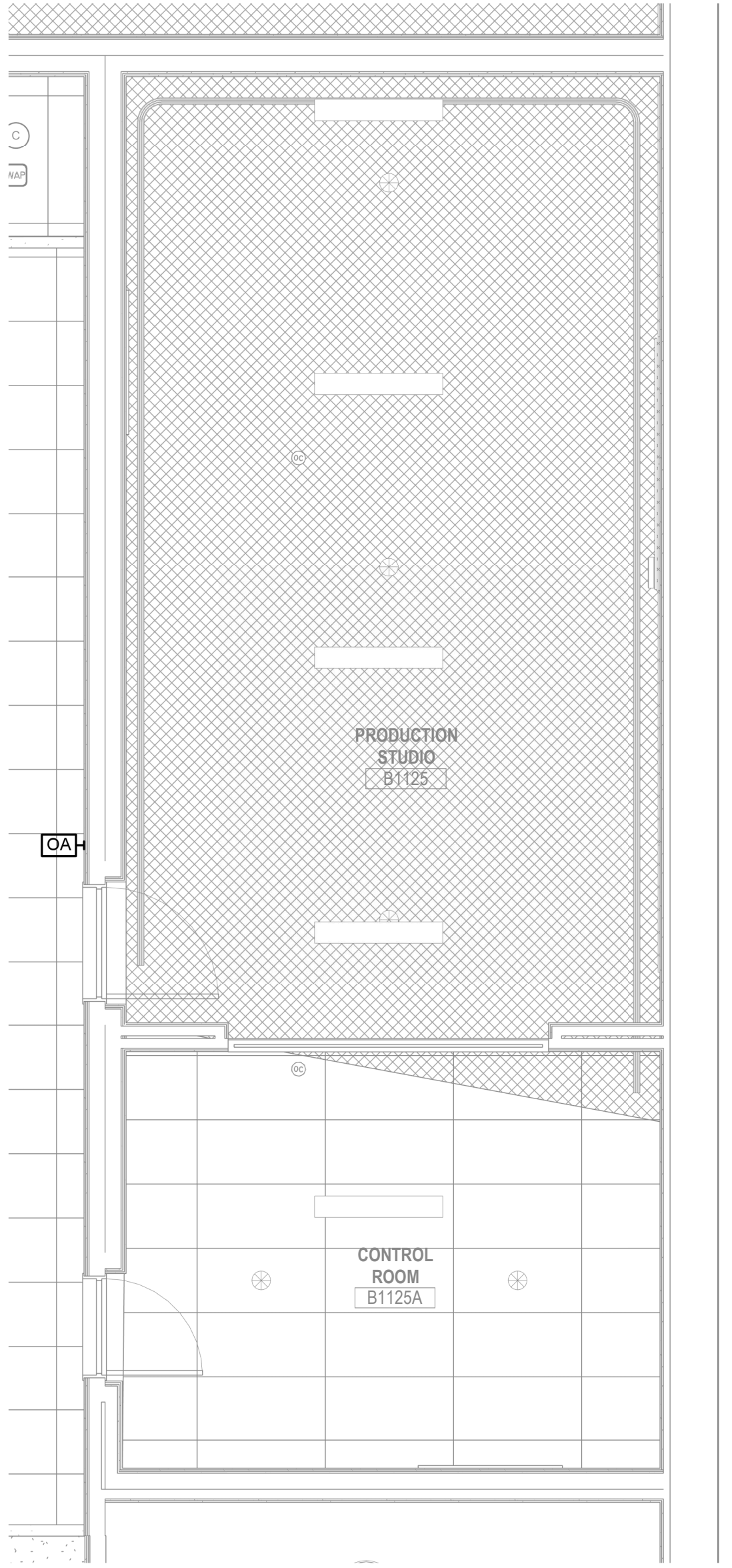
PRODUCTION STUDIO 1125 & CONTROL ROOM 1125A - ENLARGED RCP - ADDITIVE BID ALTERNATE (RECORDING STUDIO) ④ 1/4" = 1'-0"
