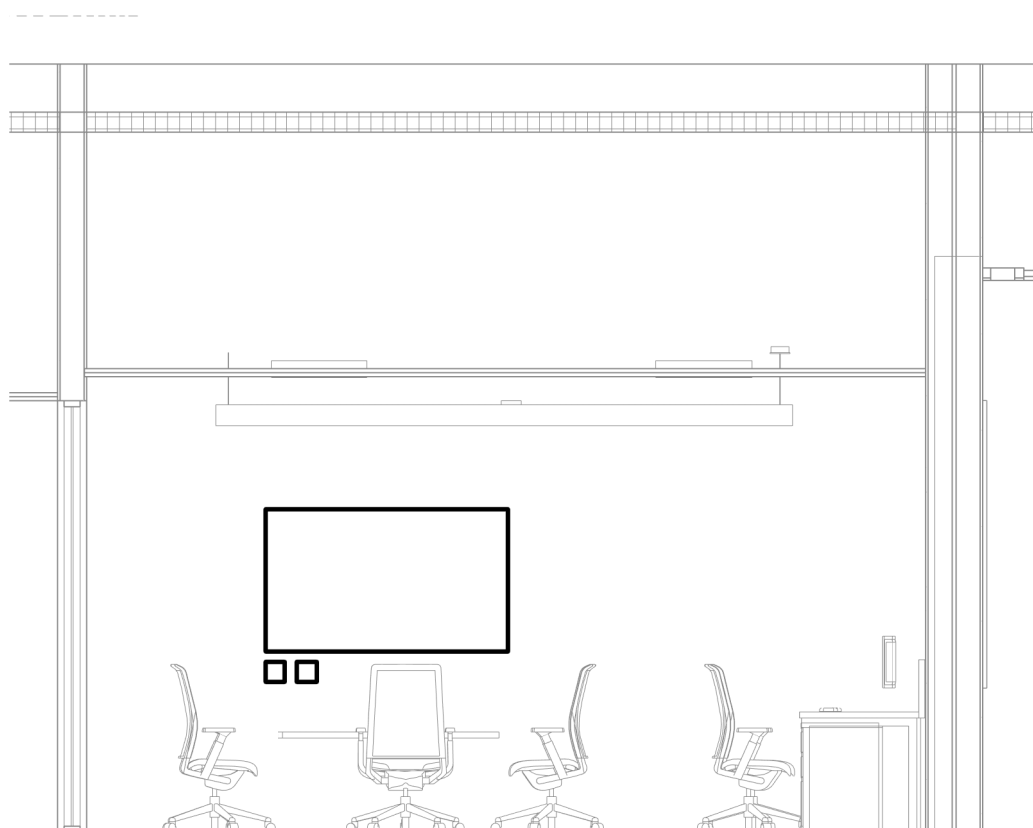
13 FACILITY MANAGER OFFICE B1336 - WEST ELEVATION 1/4" = 1'-0"
