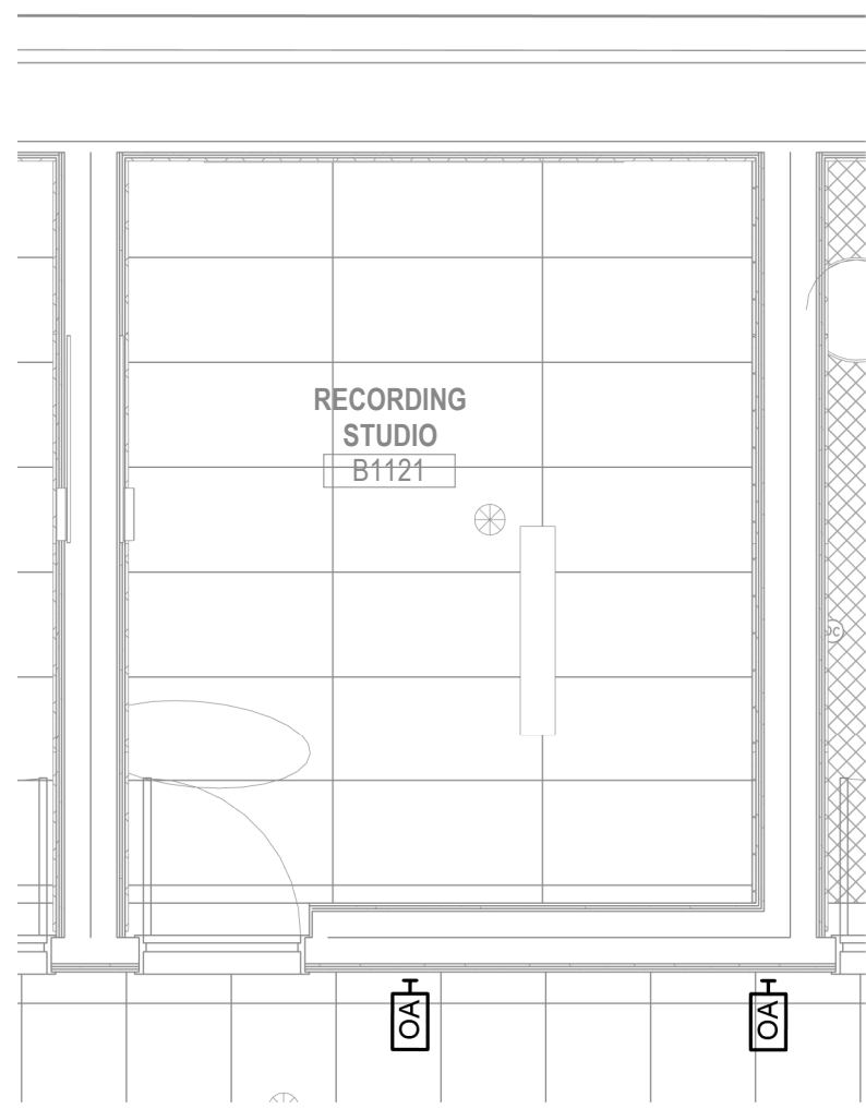
11 RECORDING STUDIO B1121 - ENLARGED RCP - ADDITIVE BID ALTERNATE (RECORDING STUDIO) 1/4" = 1'-0"
