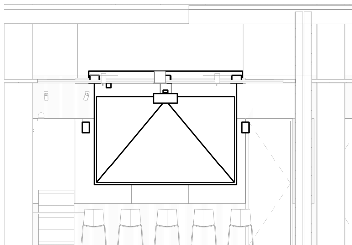
3 CLASSROOM 30 SEATS B1015 - SOUTH ELEVATION 1/4" = 1'-0"
