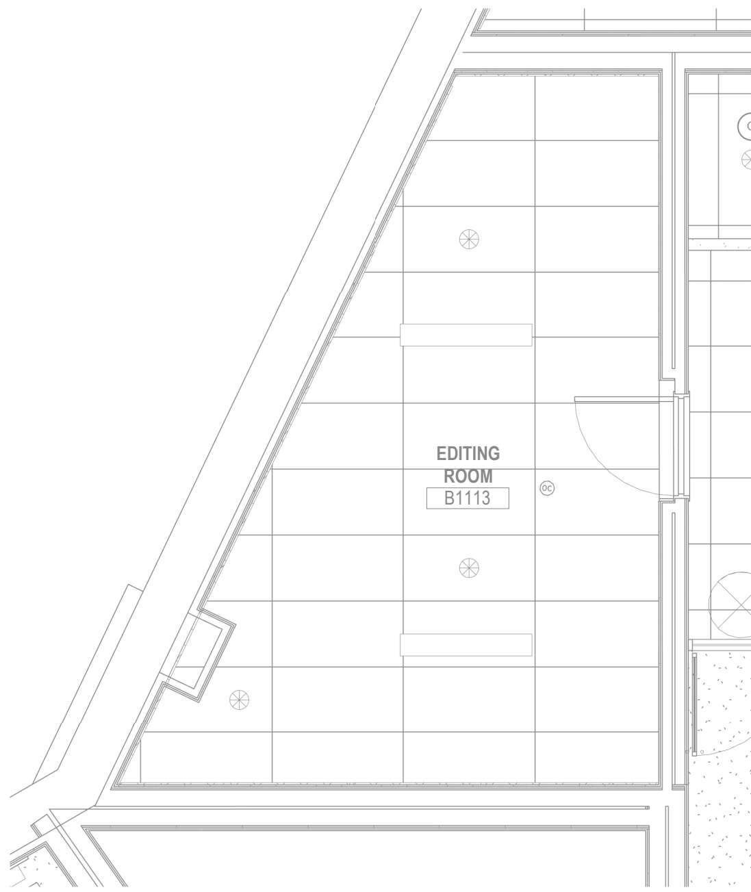
EDITING ROOM B1113 - ENLARGED RCP - ADDITIVE BID ② ALTERNATE (RECORDING STUDIO) 1/4" = 1'-0"
