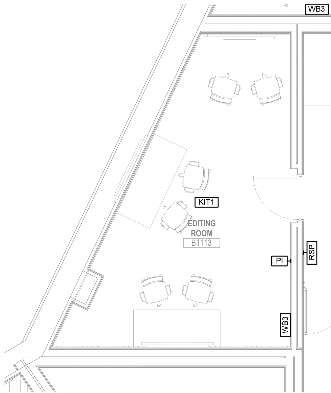
EDITING ROOM B1113 - ENLARGED PLAN - ADDITIVE BID ① ALTERNATE (RECORDING STUDIO) 1/4" = 1'-0"
