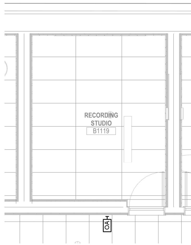
7 RECORDING STUDIO B1119 - ENLARGED RCP - ADDITIVE BID ALTERNATE (RECORDING STUDIO) 1/4" = 1'-0"
