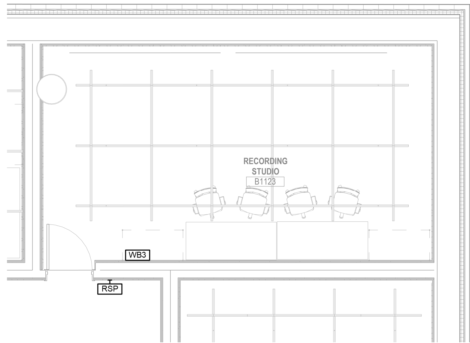
RECORDING STUDIO B1123 - ENLARGED PLAN - ADDITIVE ⑤ BID ALTERNATE (RECORDING STUDIO) 1/4" = 1'-0"
