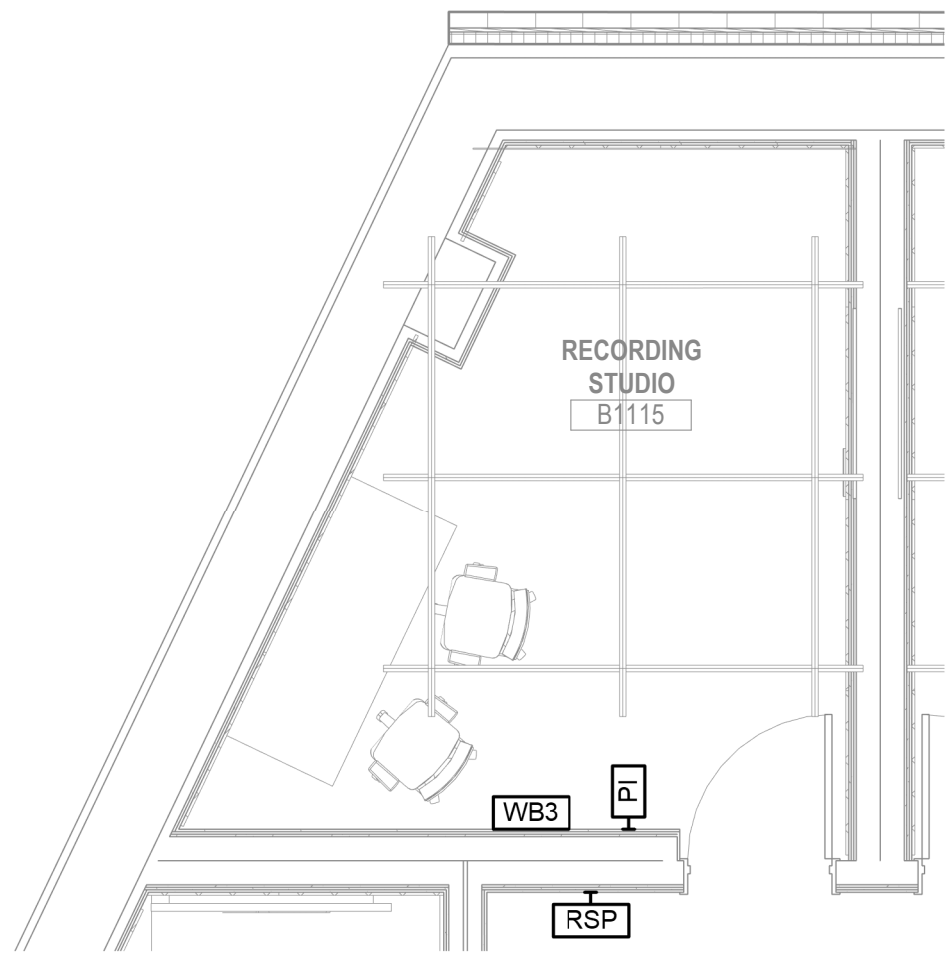
4 RECORDING STUDIO B1115 - ENLARGED PLAN - ADDITIVE BID ALTERNATE (RECORDING STUDIO) 1/4" = 1'-0"
